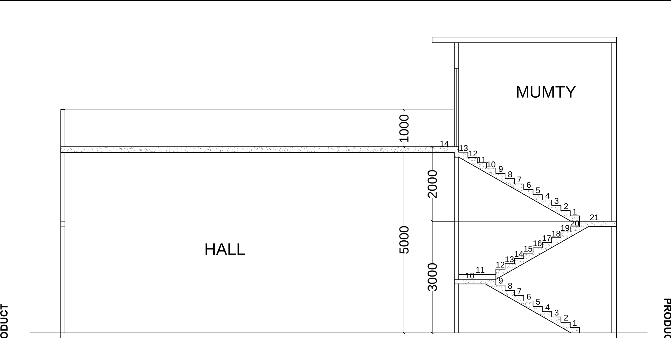
SECTION -AA
