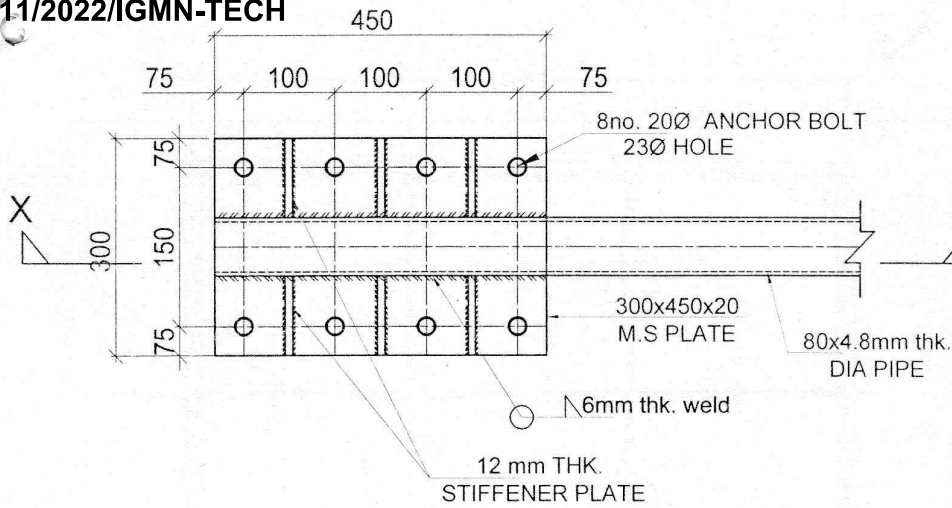
TOP PLAN PLATE & COLUMN JUNCTION DETAIL - ①
