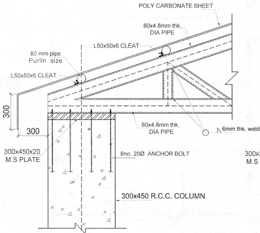
SECTION - X - X
