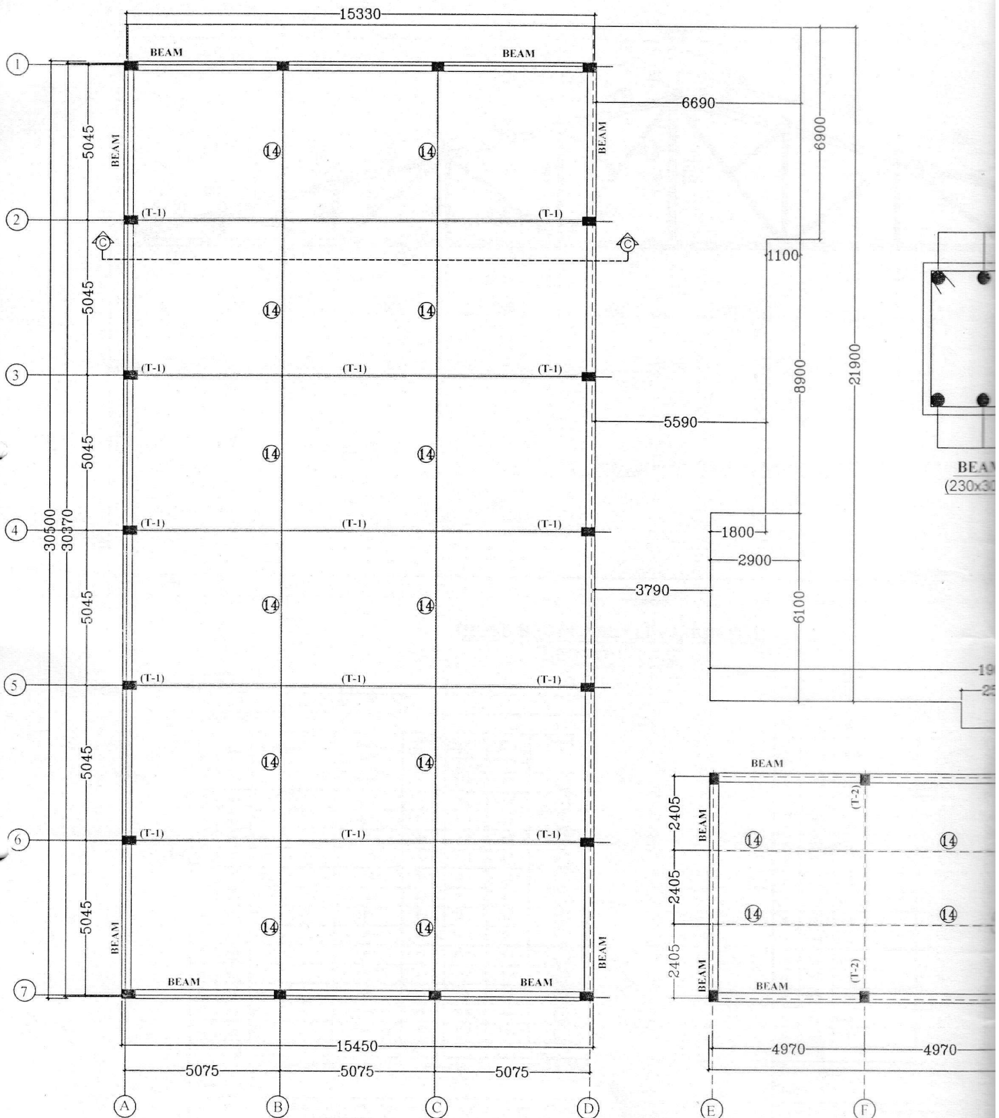
TRUSS(T-1) BOTTOM X-BRACING PLAN
